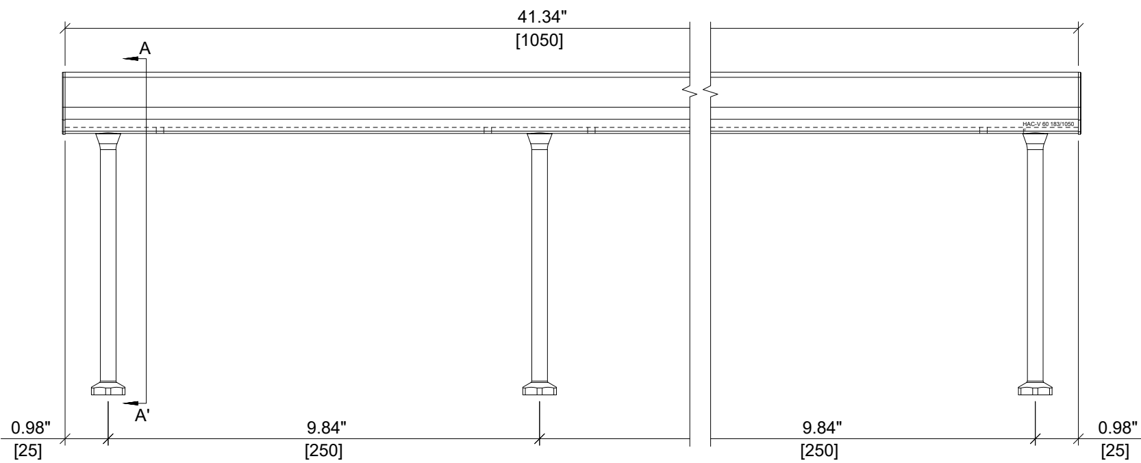
ELEVATION VIEW
