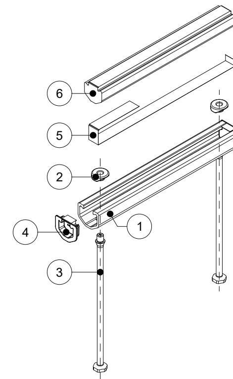
ISOMETRIC VIEW
