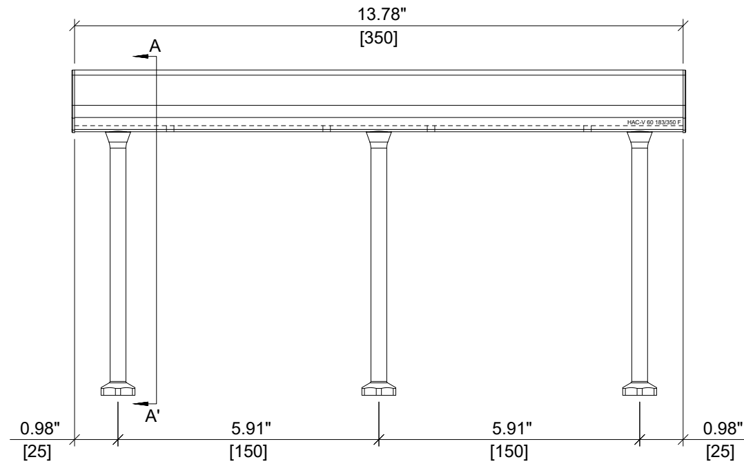
ELEVATION VIEW
