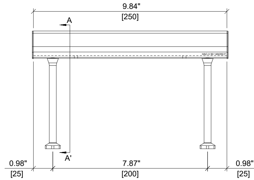
ELEVATION VIEW
