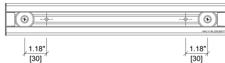
PLAN VIEW
