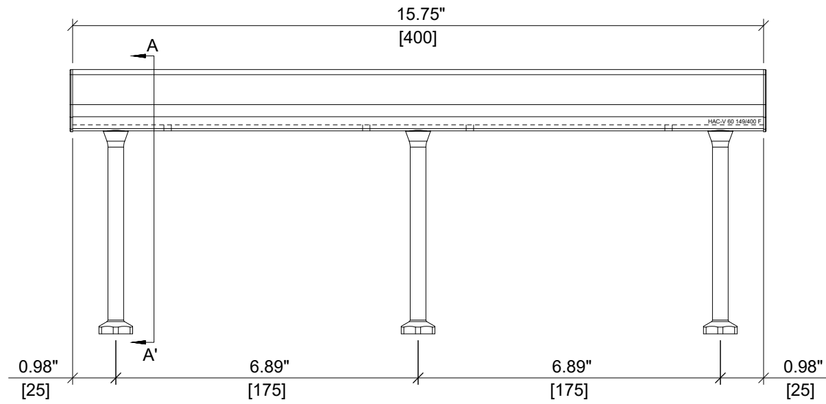
ELEVATION VIEW
