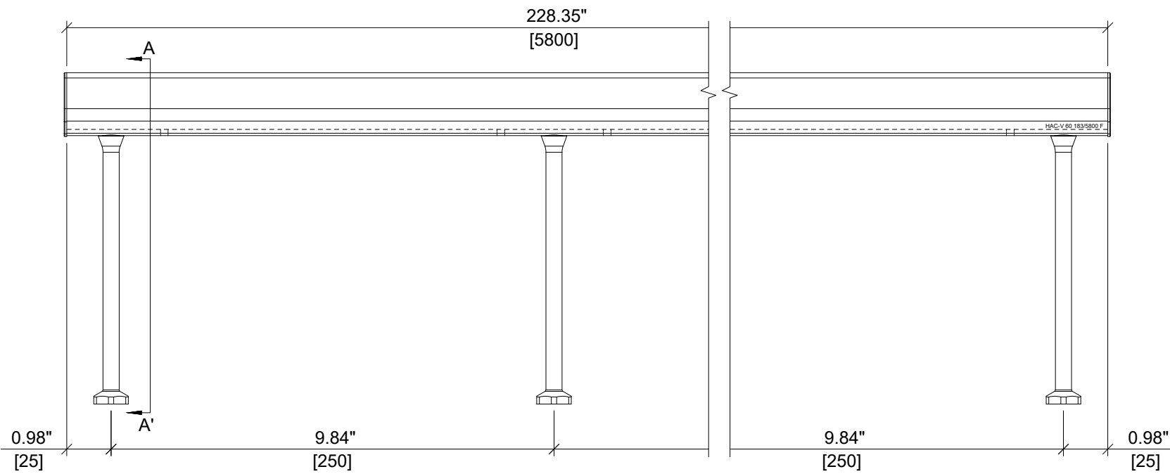
ELEVATION VIEW
