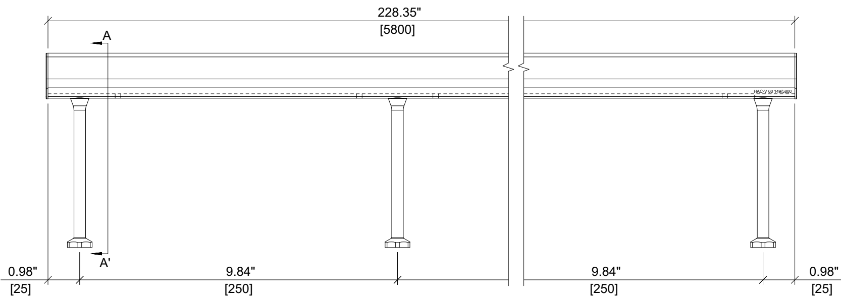
ELEVATION VIEW
