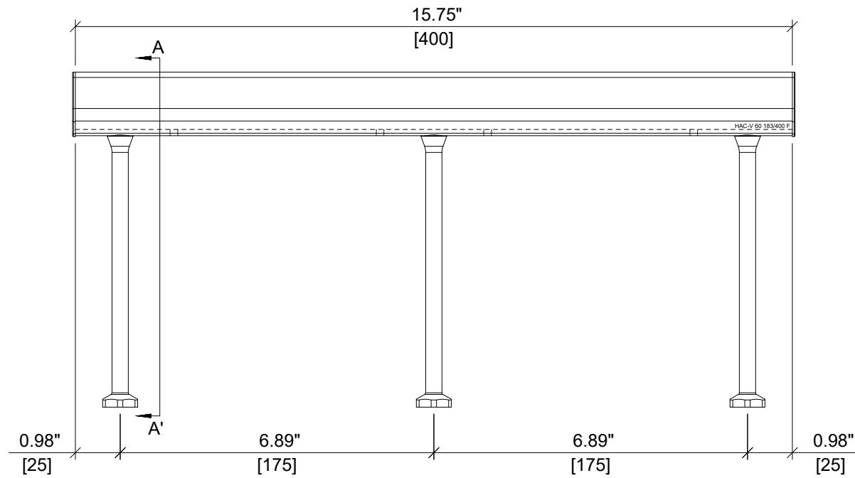
ELEVATION VIEW
