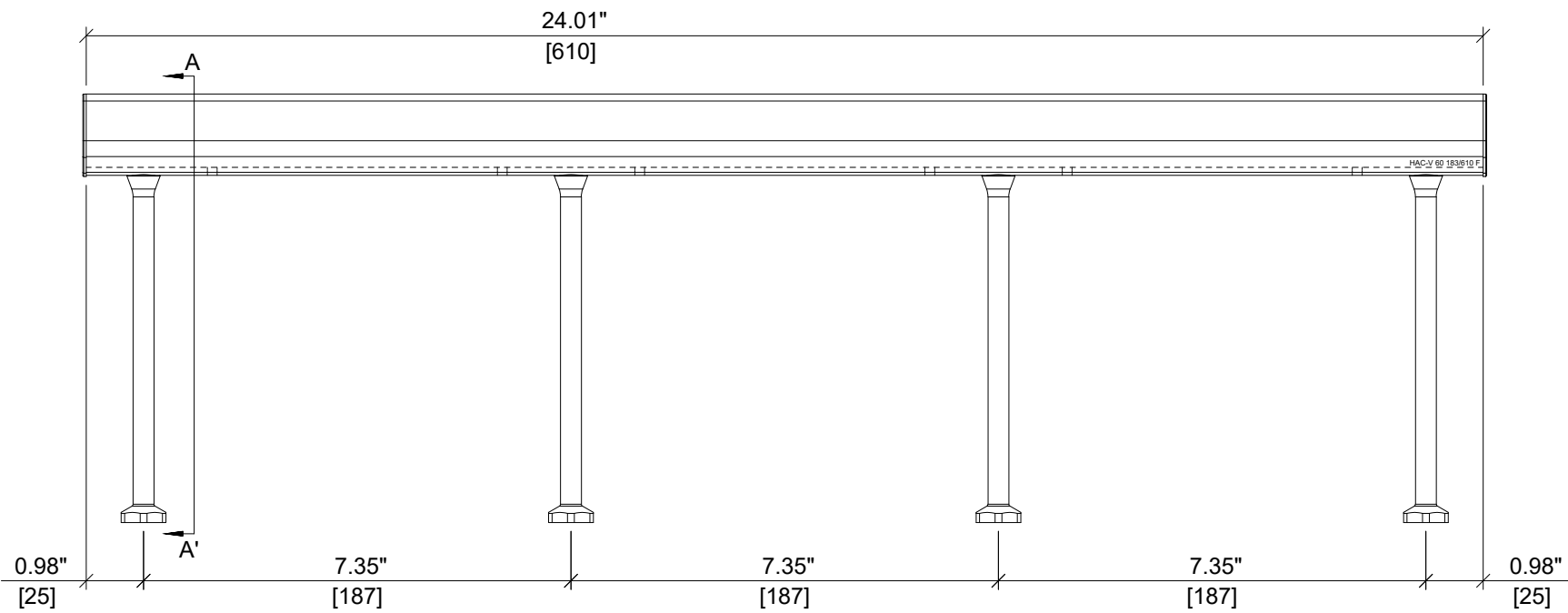
ELEVATION VIEW
