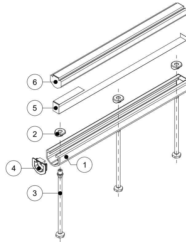
ISOMETRIC VIEW
