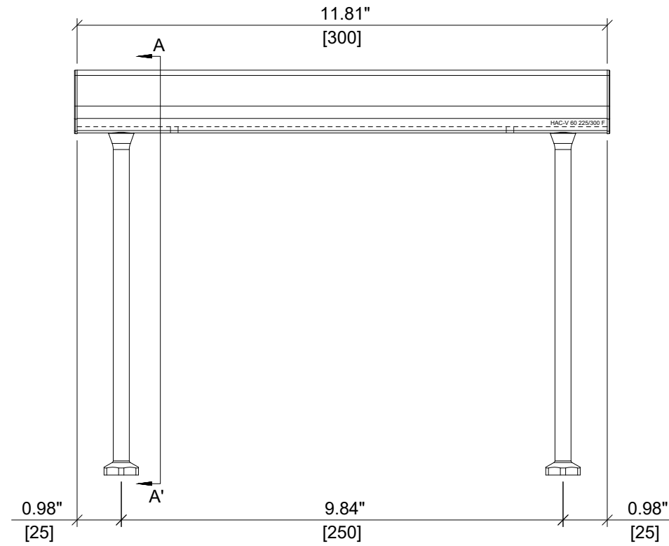
ELEVATION VIEW
