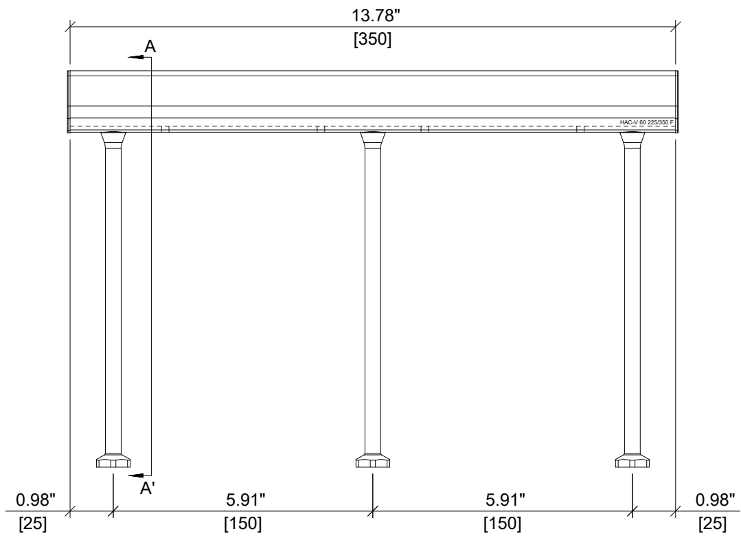
ELEVATION VIEW
