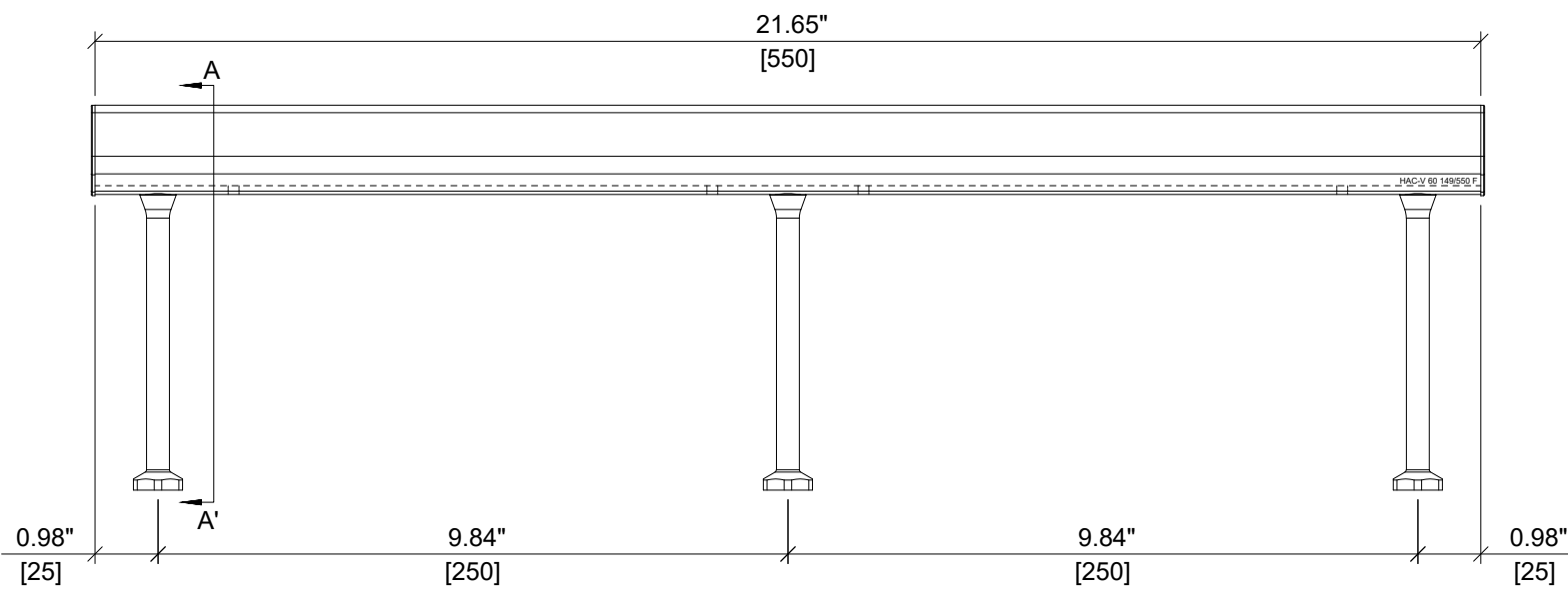
ELEVATION VIEW
