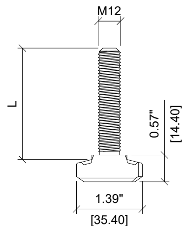
ELEVATION VIEW
