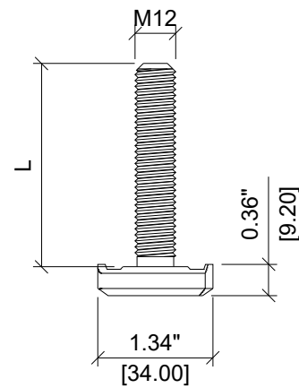
ELEVATION VIEW
