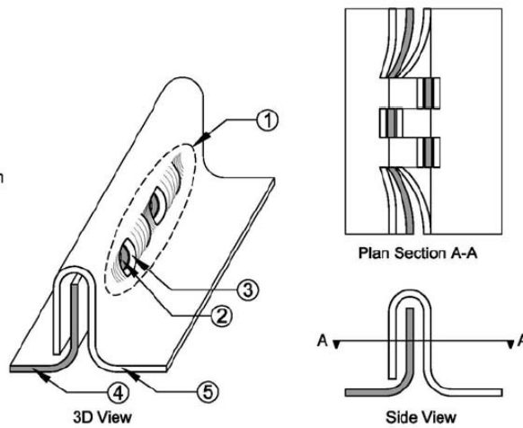
4e. Verc VSC 2 Connection
