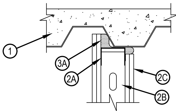
SECTION A-A CONFIGURATION B
