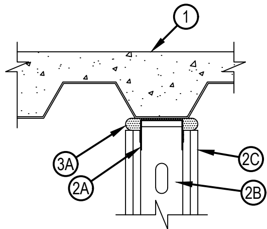
SECTION A-A CONFIGURATION A
